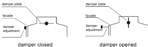
Fig. 5. The example of the damper adjustment
